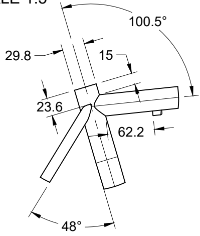
DETAIL B SCALE 1:5
