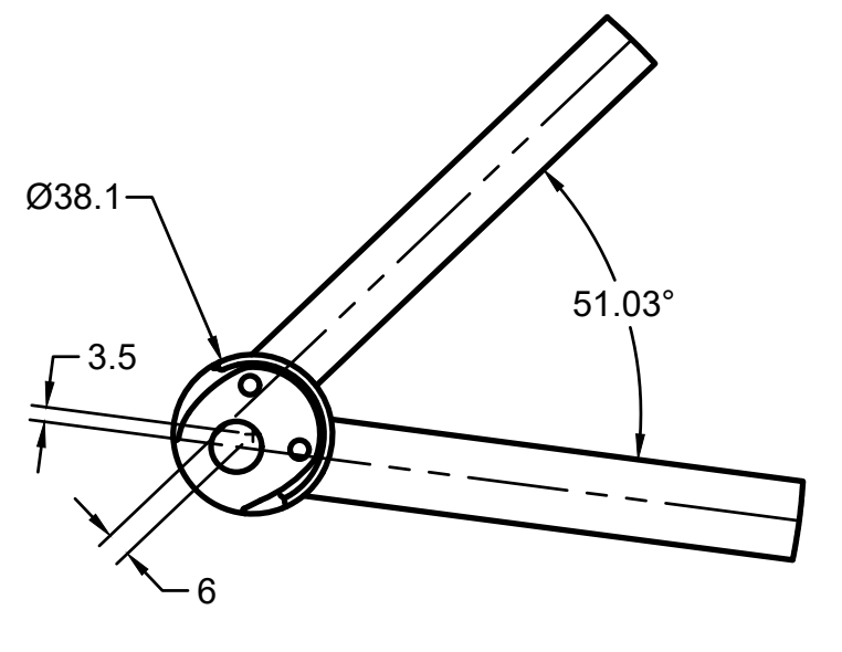
DETAIL D SCALE 1:2
